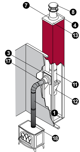
Through-the-Wall
