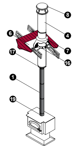
Cathedral Ceiling
