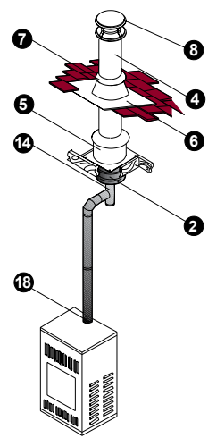
Oil Furnace
